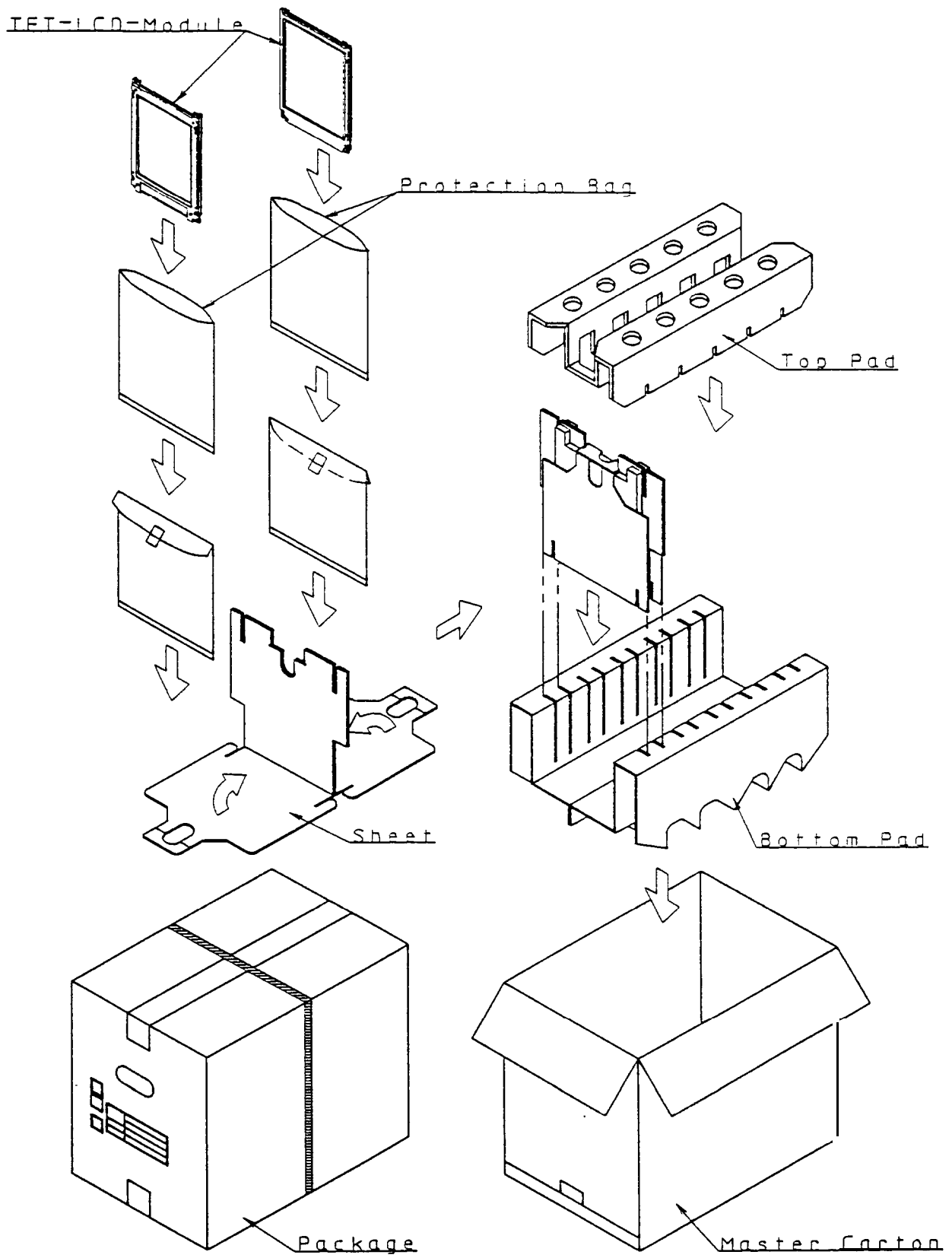
Fig. 4 Packing form
